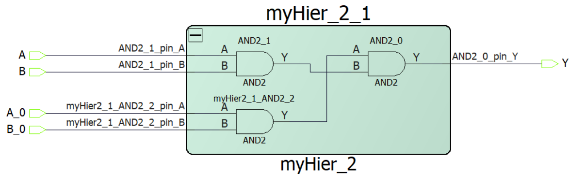
Figure 8-5. Top-Level Design—Expanded
