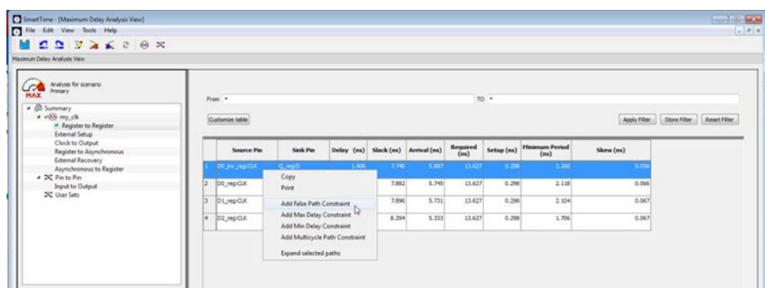
Figure 10-31. Right-Clicking Add False Path Constraint
