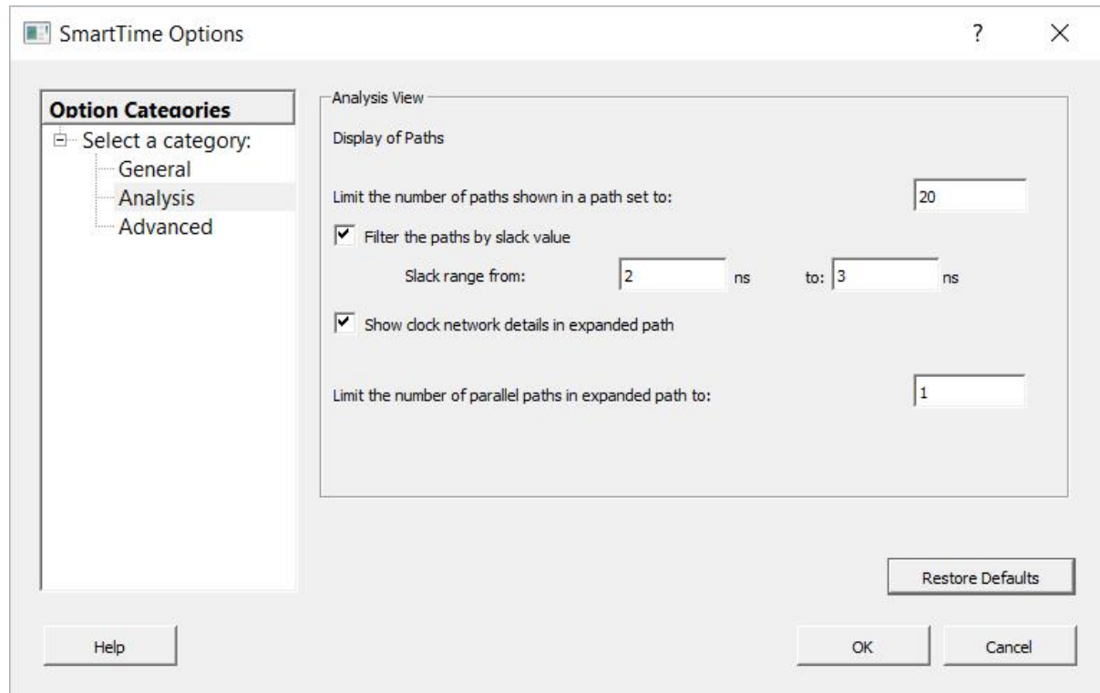
Figure 4-3. SmartTime Options Dialog Box—Analysis Settings
