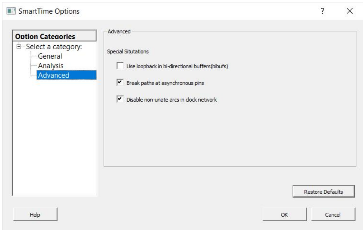
Figure 4-4. SmartTime Options Dialog Box—Advanced Settings
