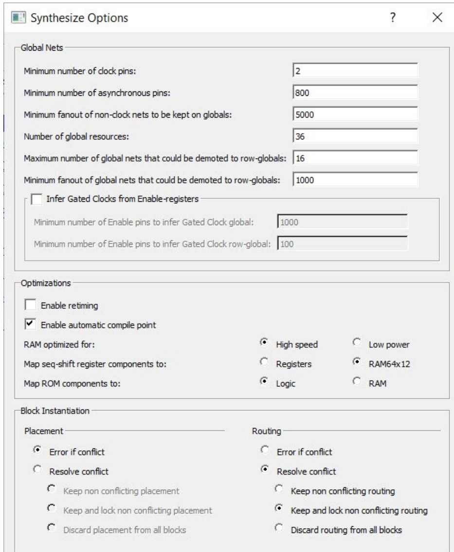
Figure 8-1. Synthesis Options Dialog Box
