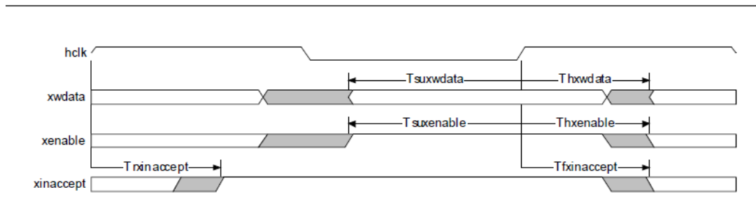
Figure 2-3. Crypto DXI Signal Waveform
