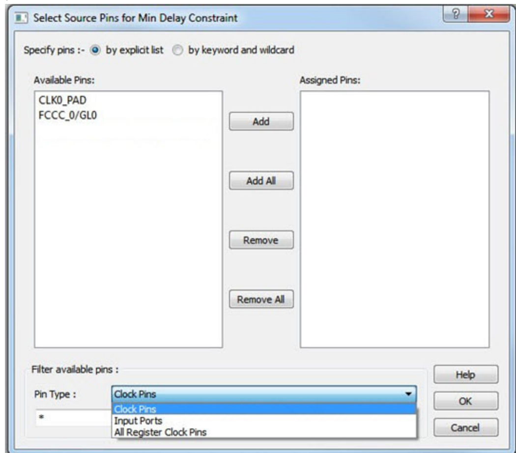
Figure 20 · Select Source Pins for Min Delay Constraint Dialog Box
