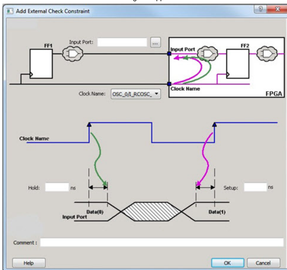
Figure 11 - Add External Check Constraint Dialog Box
