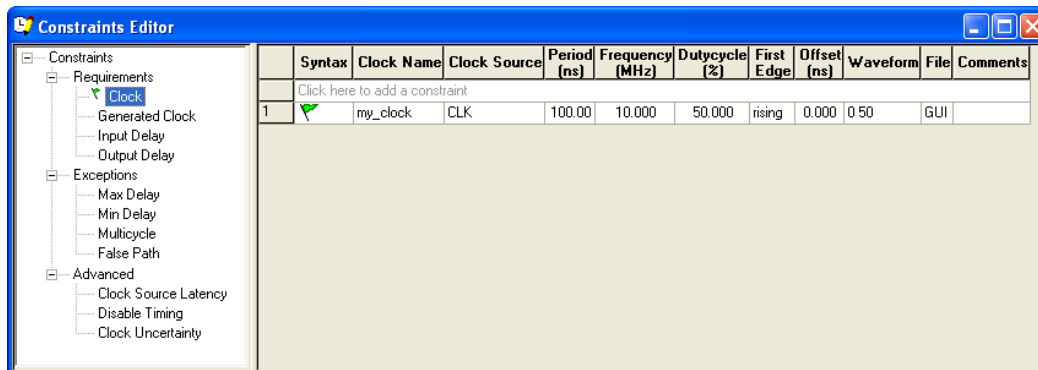
Figure 67 · Timing Constraint View
