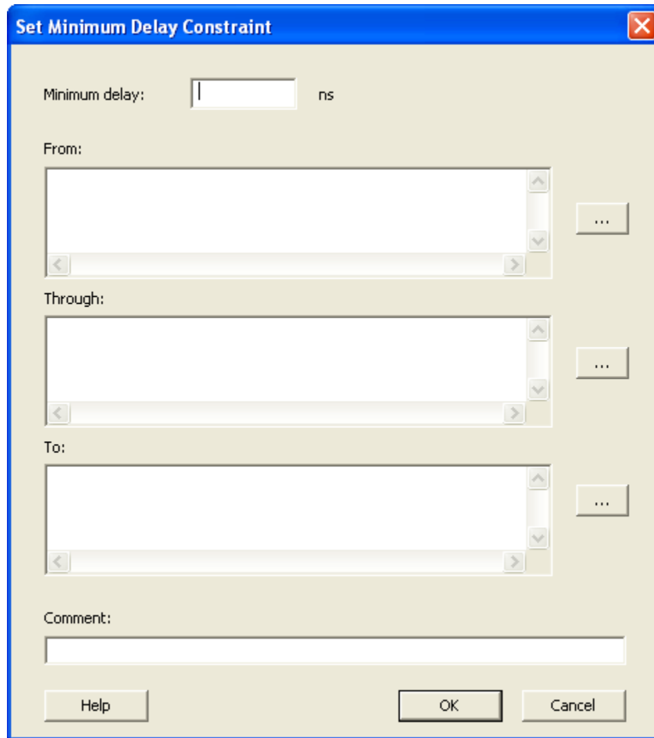
Figure 59 · Set Minimum Delay Constraint Dialog Box
