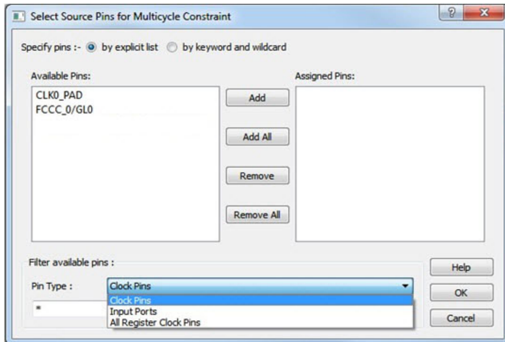
Figure 28 · Select Source Pins for False Path Constraint Dialog Box
