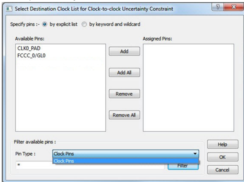
Figure 38 · Select Destination Clock List for Clock-to-Clock Uncertainty Dialog Box
