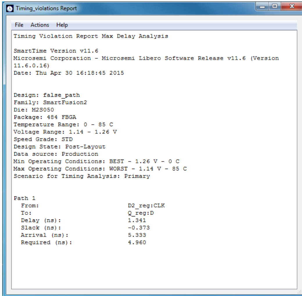
Figure 24 · Timing Violations Report
